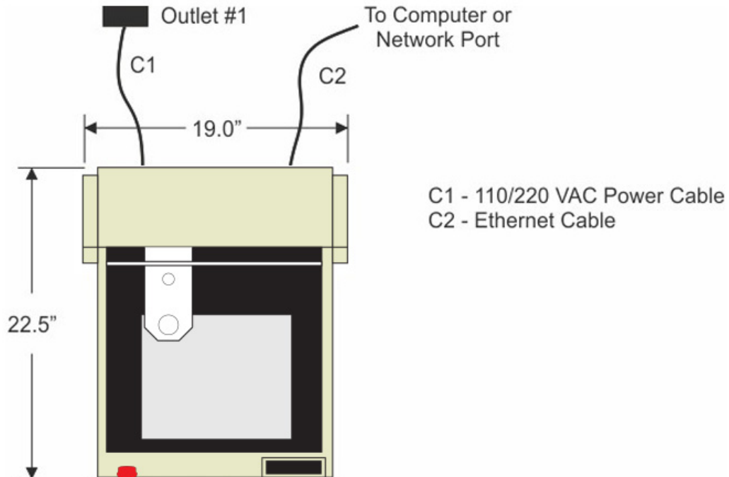
Vision VE810 Engraver Installation Layout
