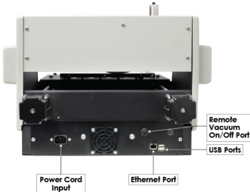
VE810 (rear view)
